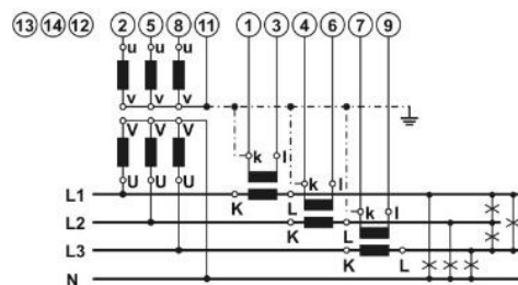
Three-phase – four-wire connection with unbalanced load
