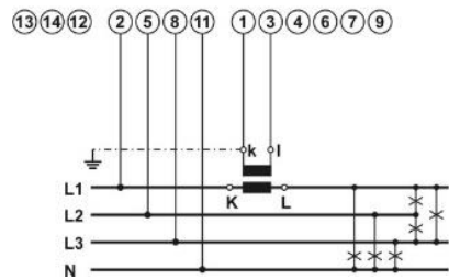
Three-phase – four-wire connection with balanced load
