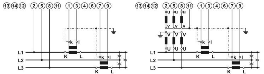
Three-phase – three-wire connection with unbalanced load
