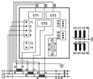
4u – four-wire, non-uniform load
