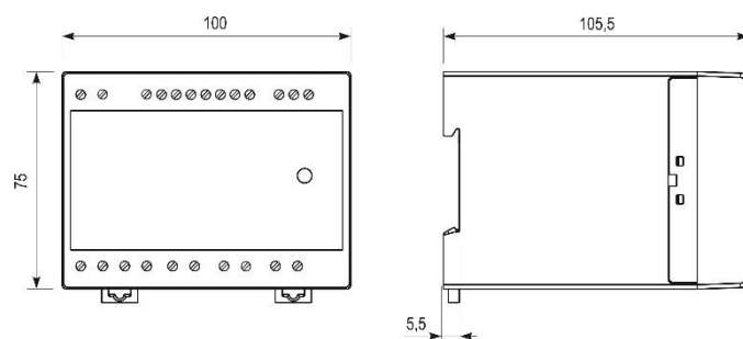
Dimensions for MT440
